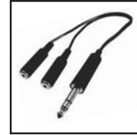
35-591 One 1/4" stereo plug to two 3.5mm stereo jacks, shielded. 10" long.
