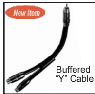
35-525-MZ Buffered "Y" Cable RCA male to dual RCA females. Multi-Zone "Y" adapter. Some A/V receivers will short the source signals when the unit is powered off. This adapter prevents this from occurring by using passive circuitry to prevent distortion and signal loss. 8mm OFC cable w/ high quality gold plated connectors 6" in length.
