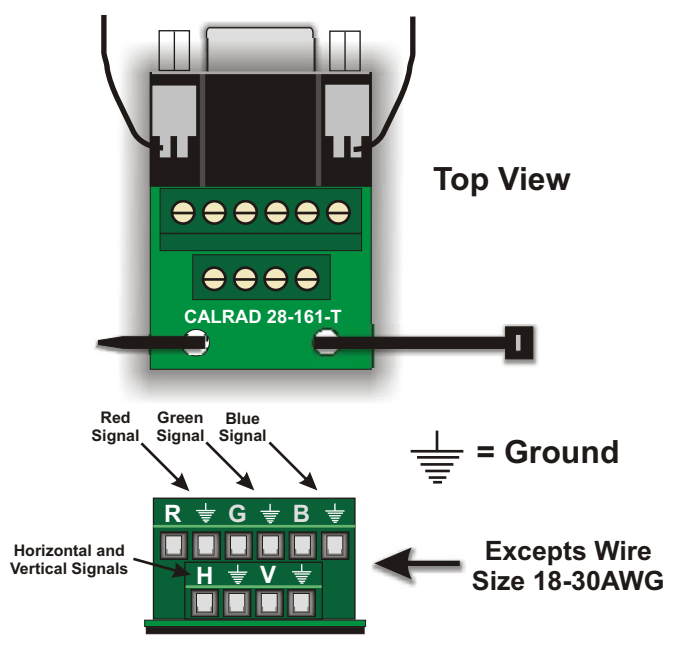
Diagram 1A. Terminal Hookup
